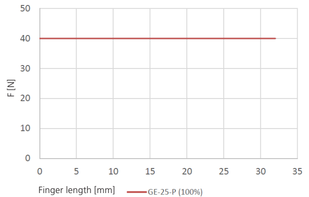
Gripping force diagram (GE-25-P 100%)
